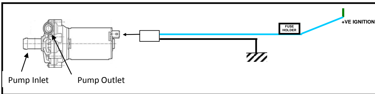
Figure 3: Wiring diagram for “CONTINUOUS EBP25 ® RUNNING”.
